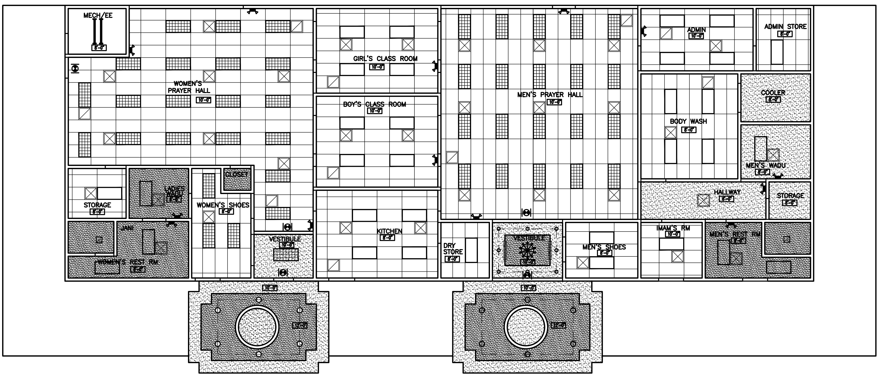
PLAN NORTH 01 REFLECTED CEILING PLAN SCALE: 1/8" = 1'-0"
