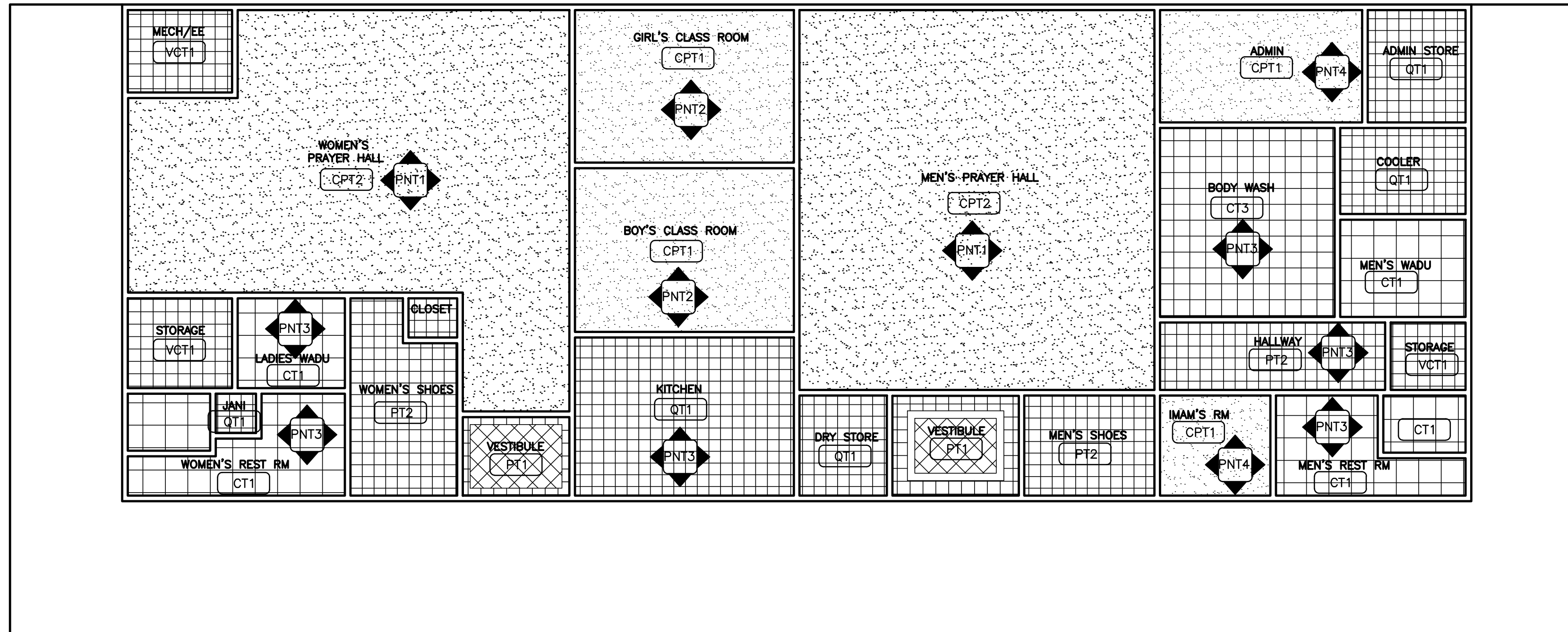
01 FINISH FLOOR PLAN SCALE: 1/8"=1'-0" PLAN NORTH
